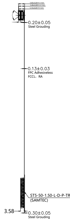
SIDE VIEW
